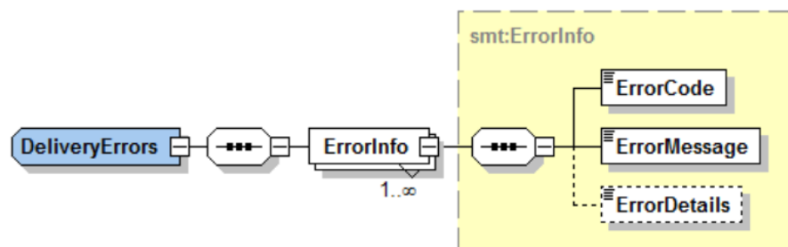
Figure 9. Record-level errors.
