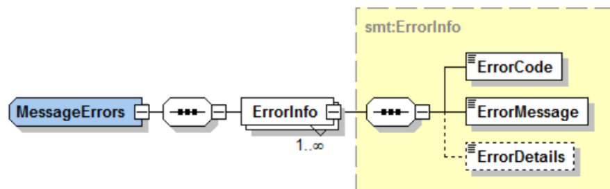
Figure 8. Message-level errors.
