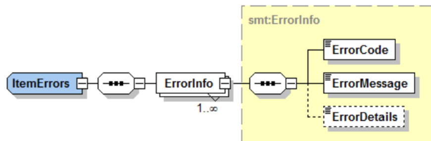
Figure 10. Item-level errors.
