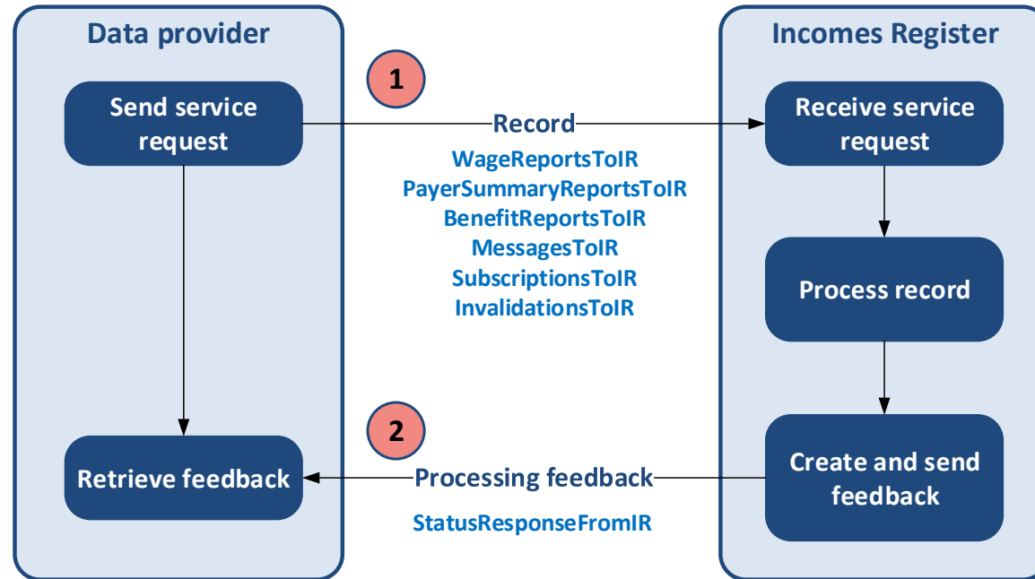
Figure 17. Submitting data via the real-time Web Service interface.
