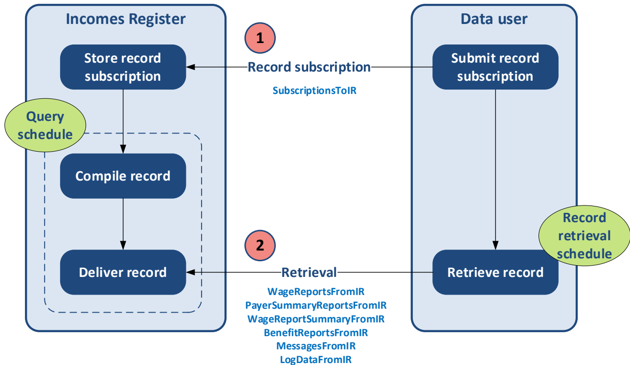
Figure 3. Distribution of data via the SFTP interface
